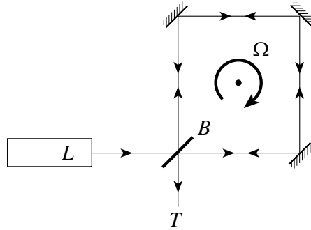
Fig. 8.10: Sagnac Interferometer used as a type of laser gyro.
