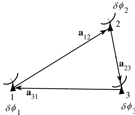
Fig. 8.5: Closure phase measurement using a triangle of telescopes.
