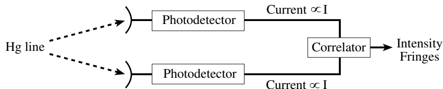
Fig. 8.12: Hanbury-Brown and Twiss Intensity Interferometer.
