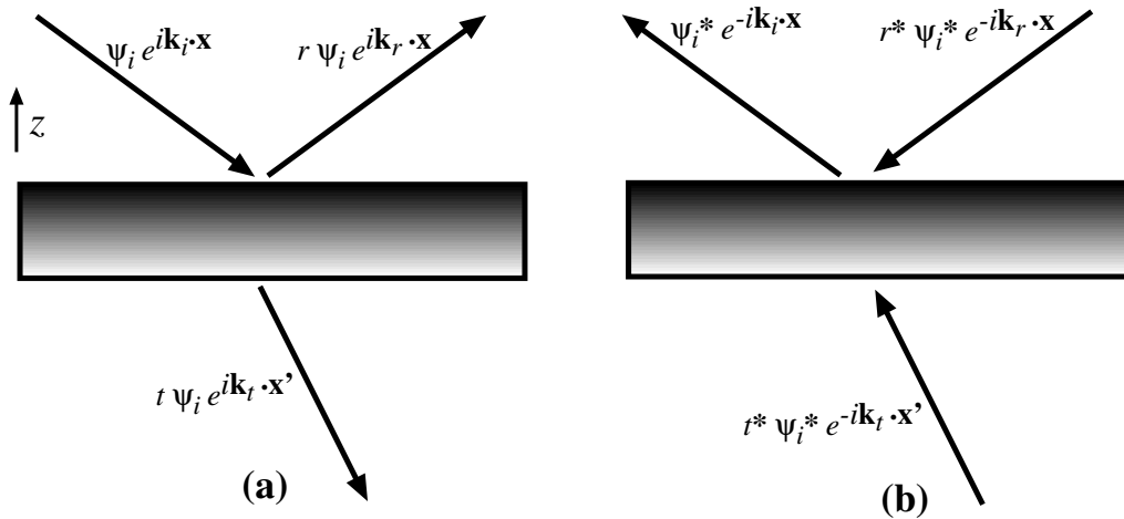
Fig. 8.9: Construction for deriving reciprocity relations for amplitude transmission and reflection coefficients.
