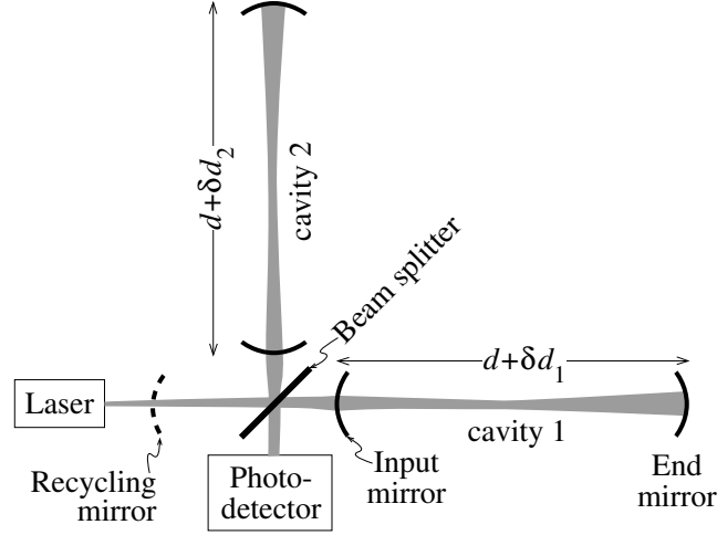
Fig. 8.11: Laser Interferometer Gravitational Wave Detector.
