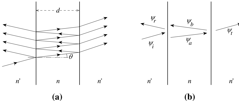
Fig. 8.6: Multiple beam interferometry using a type of Fabry-Perot Etalon.
