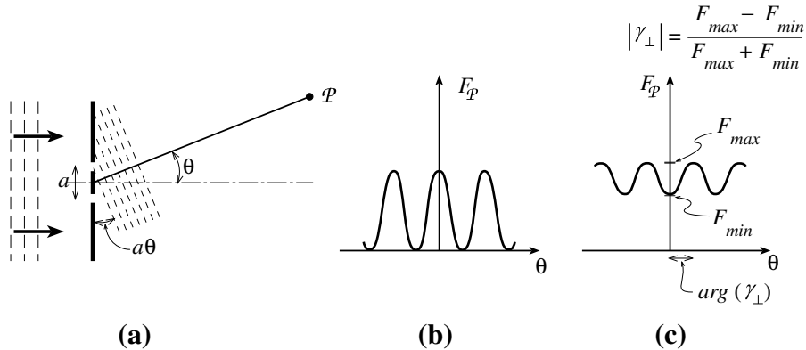
Fig. 8.1: a) Young's Slits. b) Interference fringes observed from a point source on the optic axis [Eq. (8.2)]. c) Interference fringes observed from an extended source.
