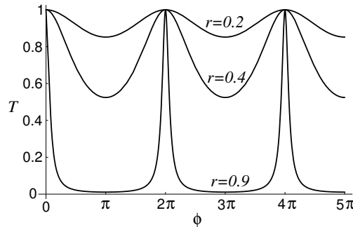
Fig. 8.8: Transmission coefficient for an etalon as a function of the phase \phi .
