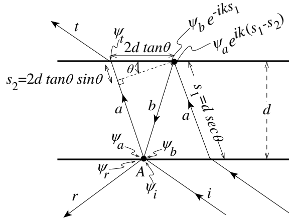
Fig. 8.7: Construction for calculating the phase differences across the slab for the two internal waves in an etalon.
