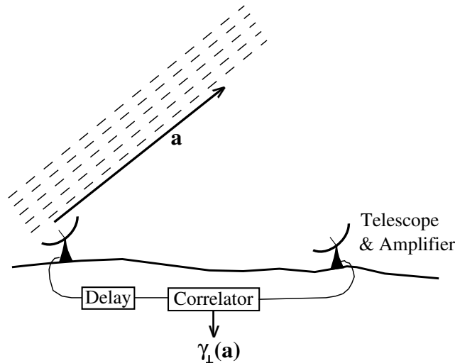
Fig. 8.4: Two Element Radio Interferometer.
