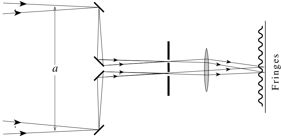
Fig. 8.2: Schematic Illustration of a Michelson Stellar Interferometer.
